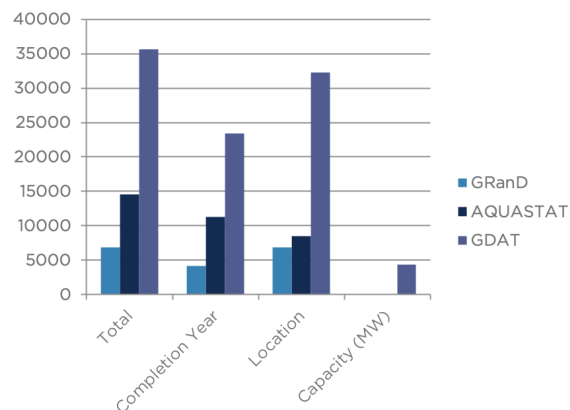
Figure 13: Number of dams with information on location, installed capacity, year of completion for AQUASTAT, GRanD, and GDAT
