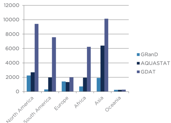
Figure 14: Total number of dams by region for AQUASTAT, GRanD, and GDAT
