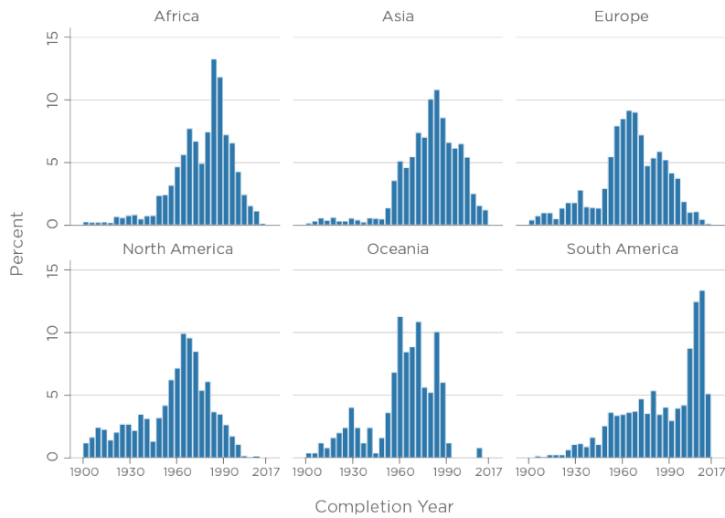
Figure 2: Distribution of dam completion year by continent
