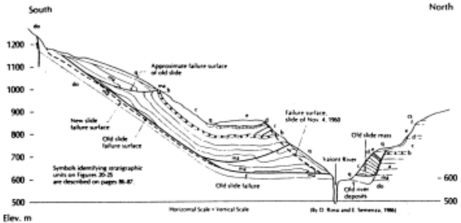
Fig. A1-2 Cross section through Vaiont Slide prior to failure (from Hendron & Patton, 1986)
